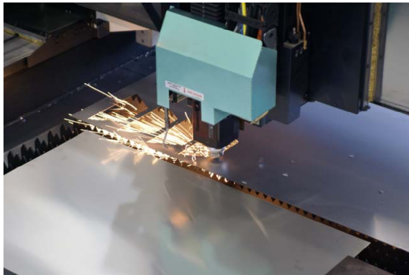
CAPTION: The new Mazak HyperGear Champion laser-cutting system with 1" cut capacity in mild steel.
